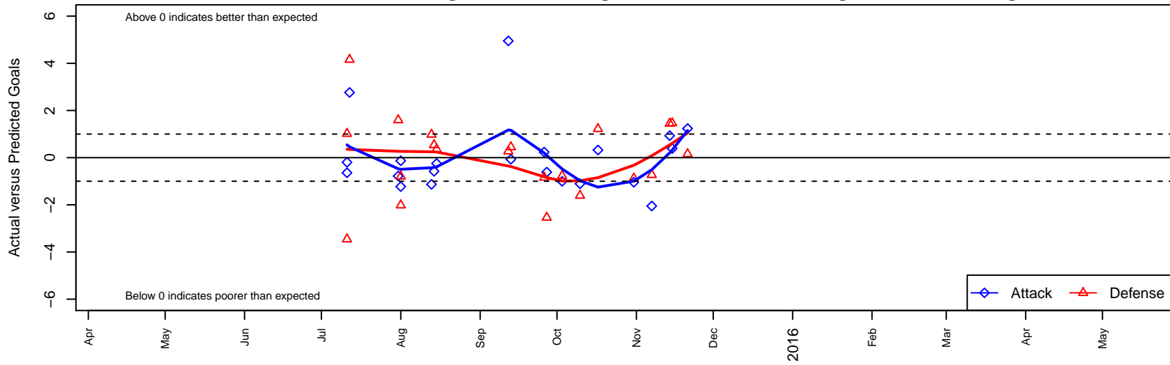
Cascade FC White G01 Dots are actual minus expected GF (blue circles) and GA (red triangles). Blue line is smoothed change in attack strength. Red is smoothed change in defense strength.
